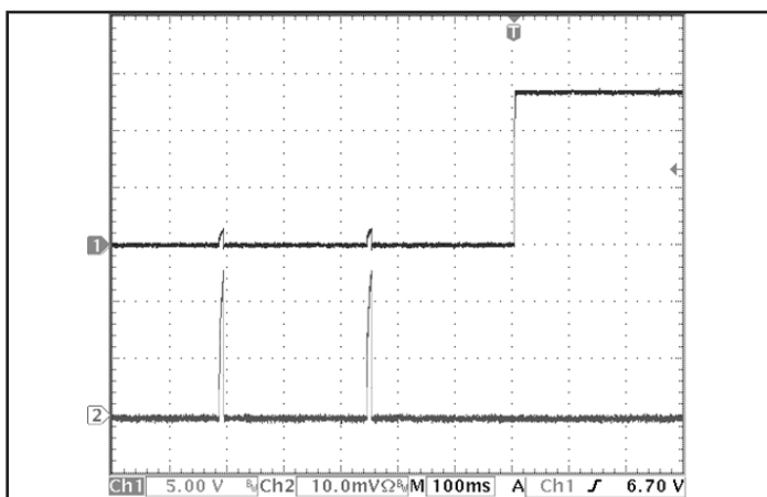
Figure 17: Rise of output voltage after the removal of a short circuit across the output terminals. R_{short} = 5 \text{ m}\Omega . Ch1: (5 V/div). Ch2: I_{out} (50 A/div). Bandwidth: 20 MHz.
