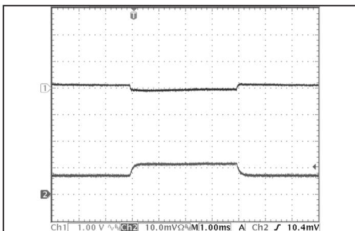
Figure 11: Output voltage response to step-change in load current (50%-75%-50% of Iout(max); dI/dt = 0.1 A/µs). Load cap: 15 µF tantalum cap and 1 µF ceramic cap. Ch 1: Vout (1 V/div), Ch 2: Iout (50 A/div).
