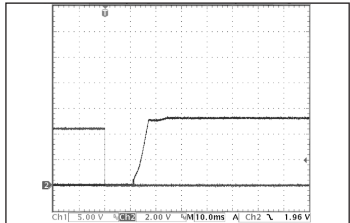
Figure 10: Turn-on transient at half load (resistive load) (10 ms/div). Load cap: 15 µF tantalum capacitor and 8 mF ceramic capacitor bank. Input voltage pre-applied. Ch 1: Vout (5 V/div). Ch 2: ON/OFF input (2 V/div).
