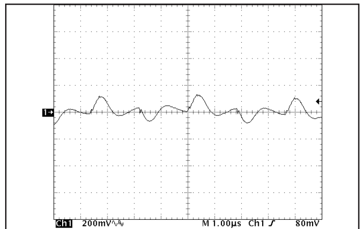
Figure 16: Output voltage ripple at nominal input voltage and rated load current (200 mV/div). Load capacitance: 1 μF ceramic capacitor and 15 μF tantalum capacitor. Bandwidth: 20 MHz. See Figure 13.
