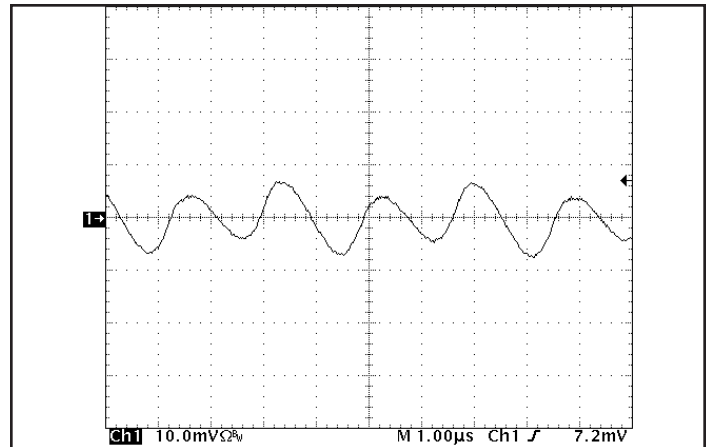
Figure 14: Input Terminal Ripple Current, i_c , at full rated output current and nominal input voltage with 10 μH source impedance and 47 μF electrolytic capacitor (200 mA/div). See Figure 13.
