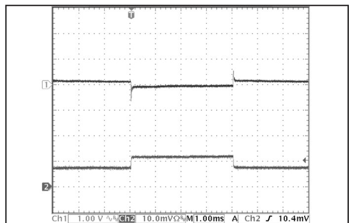
Figure 12: Output voltage response to step-change in load current (50%-75%-50% of Iout(max); dI/dt = 1 A/µs). Load cap: 15 µF, 30 mΩ ESR tantalum cap and 1 µF ceramic cap. Ch 1: Vout (1 V/div), Ch 2: Iout (50 A/div).
