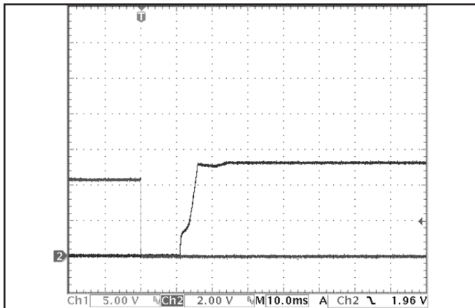
Figure 9: Turn-on transient at half load (resistive load) (10 ms/div). Load cap: 15 µF tantalum capacitor and 1 mF ceramic capacitor bank. Input voltage pre-applied. Ch 1: Vout (5 V/div). Ch 2: ON/OFF input (2 V/div).
