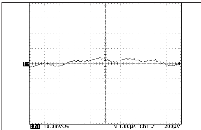
Figure 15: Input reflected ripple current, i_s , through a 10 μH source inductor, using a 47 μF electrolytic input capacitor (10 mA/div). See Figure 13.
